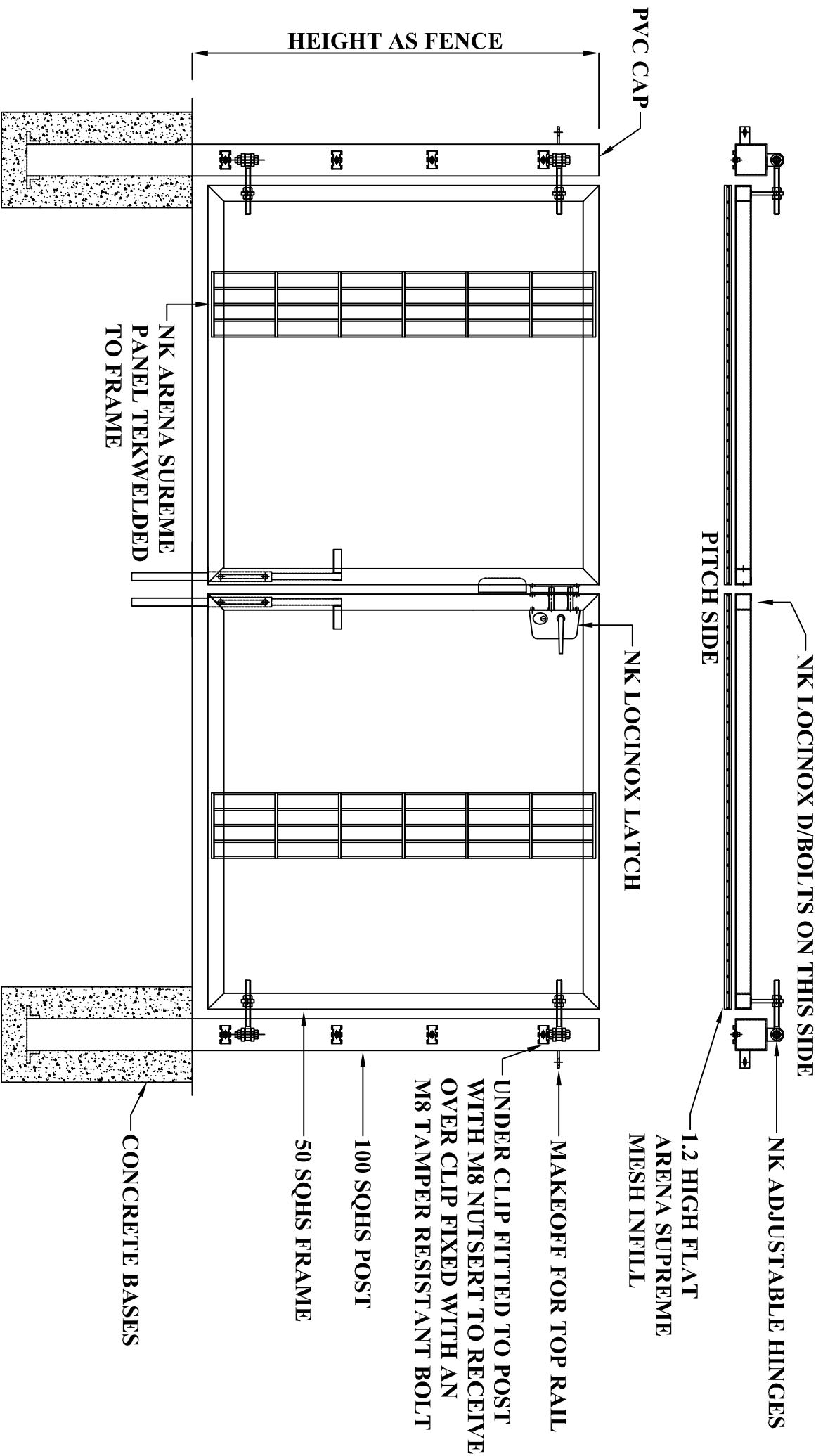
NK ARENA SPECTATOR D/L GATE - TYPICAL ELEVATION
