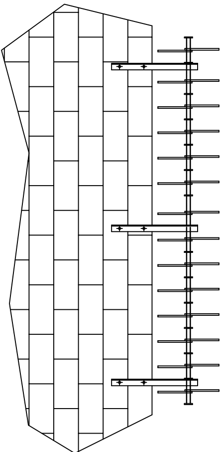
NK TOPSPIKE BOLTED TO TOP OF WALL
